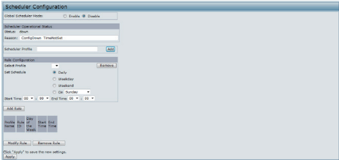
Figure 21 - Scheduler Configuration
