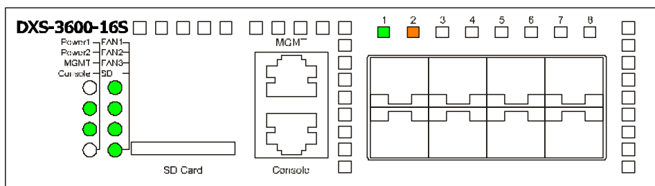
Figure 1-3 LED indicators for the DXS-3600-16S
