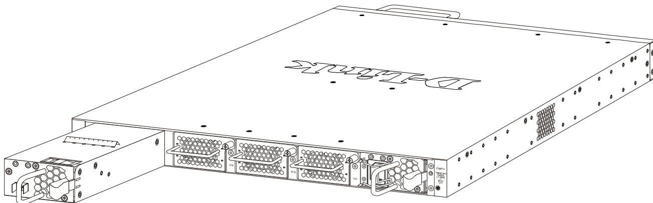
Figure 2-7 Installing a DC Power Supply Module
