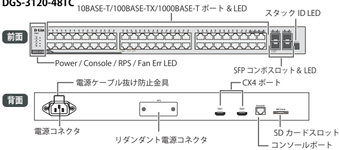
DGS-3120-48TC
