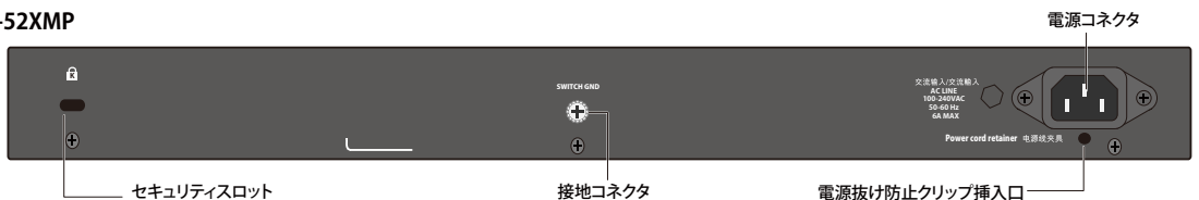
DGS-1250-52XMP
