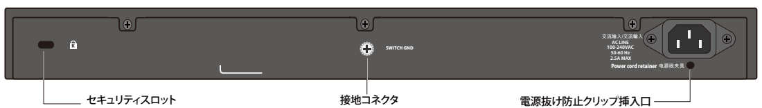
DGS-1250-52XMP
