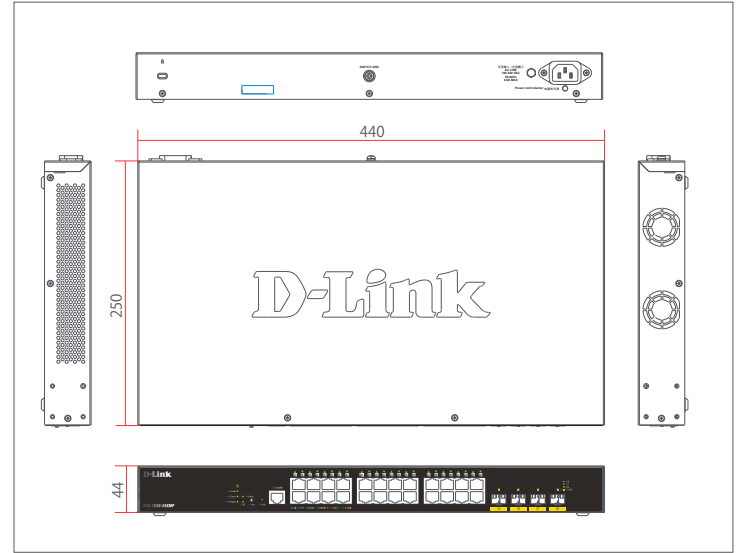
DGS-1250-28XMP
