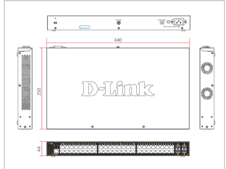
DGS-1250-52XMP
