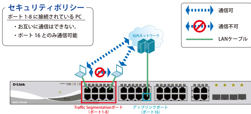
図 1-1 Traffic Segmentation (DGS-1210-28)
