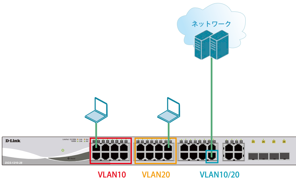
図 9-5 VLAN (DGS-1210-28)
