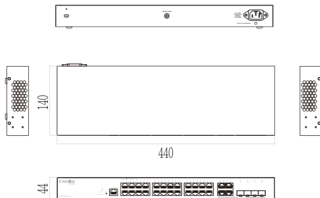
DBS-2000-28
