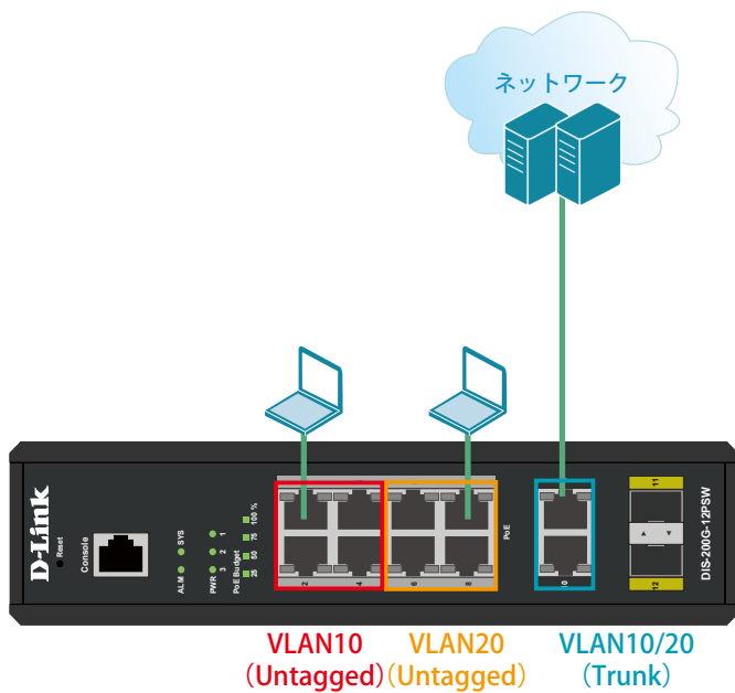
図 16-5 VLAN (DIS-200G-12PSW)
