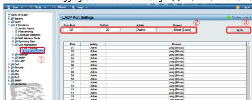
図 1-15 LACP (Active) (DES-1210-28)
