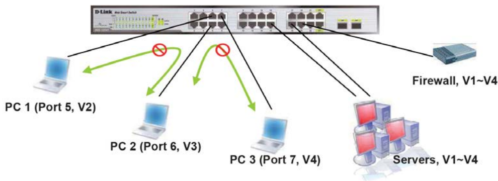
図 5-41 Asymmetric VLAN
