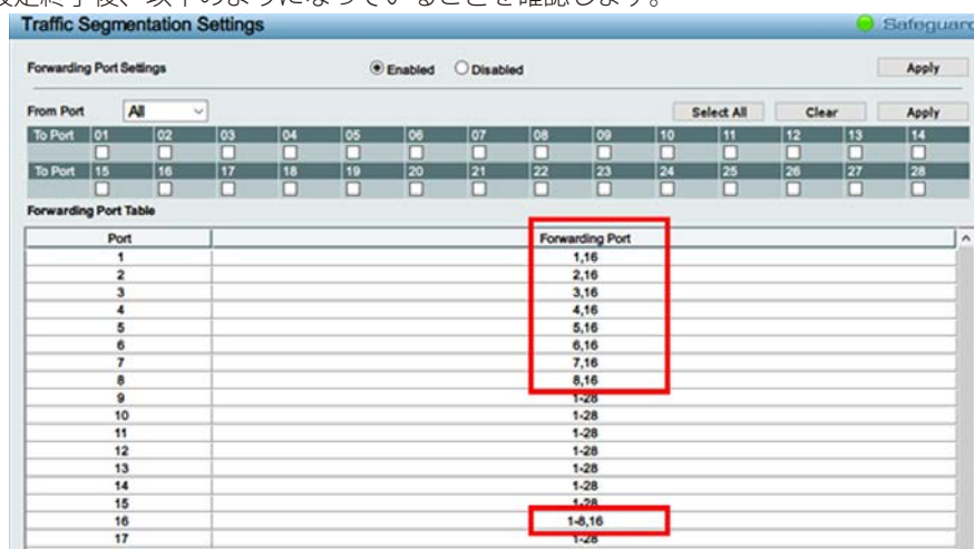
図 1-3 Traffic Segmentation Settings (DES-1210-28)
